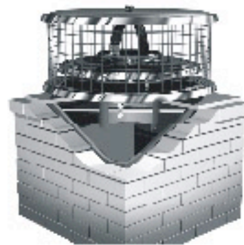
Masonry adapter required for masonry chimneys
